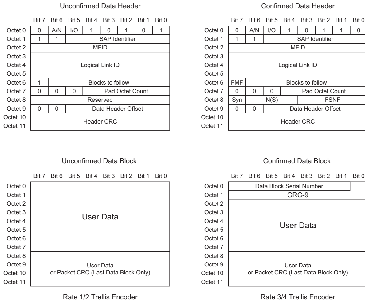
Figure 4-11: Unconfirmed and Confirmed Header and Data Blocks
